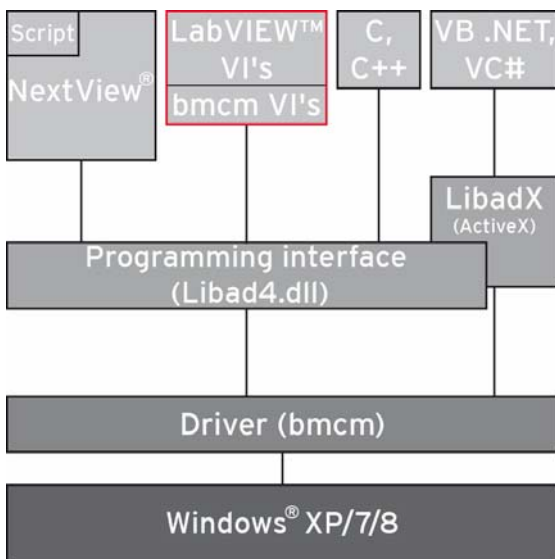
Functional diagram
