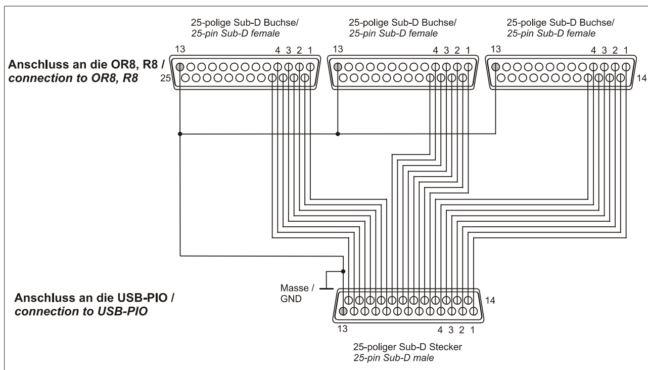
Interfacing example
