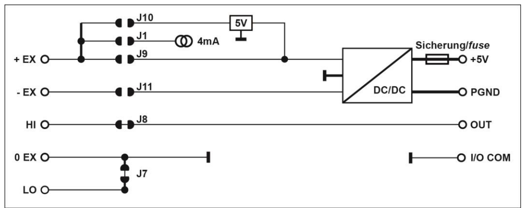
Function diagram
